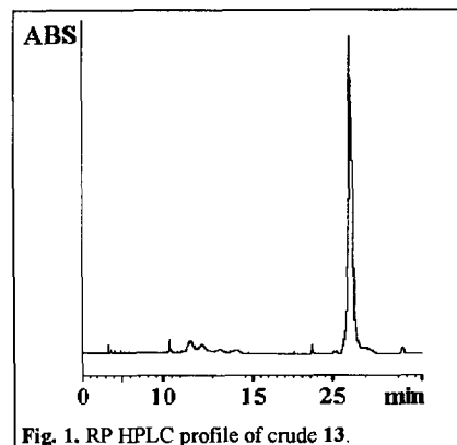
Fig. 1. RP HPLC profile of crude 13 .
